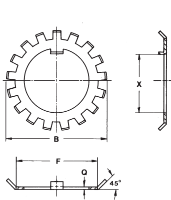
Figure 2 - LOCKWASHERS
