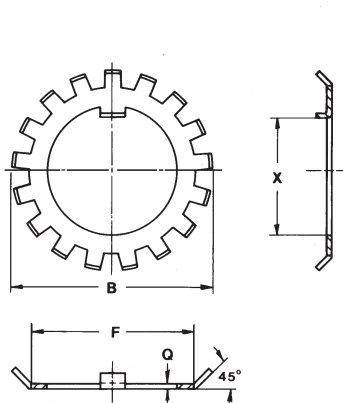
Figure 2 - LOCKWASHERS
